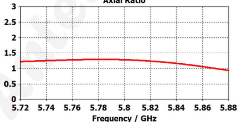
Axial Ratio
